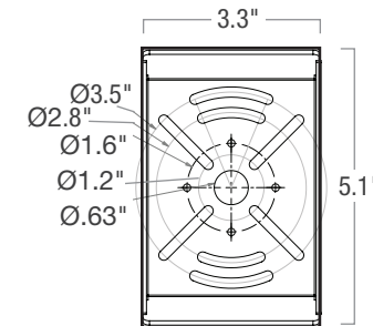
Wall Mount J-Box Mounting Bracket (included)
