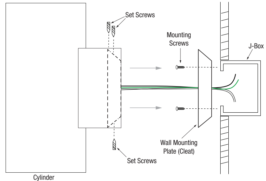
Wall Mount J-Box Mounting Bracket (included)
